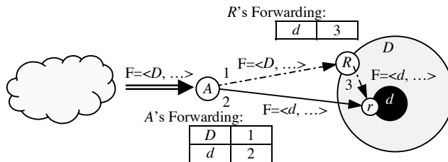
Figure 9: Conflicting SAVE updates at router r
