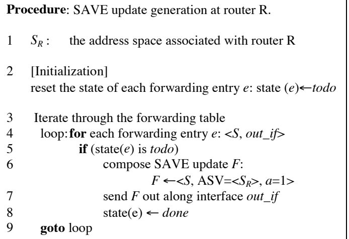
Figure 4: SAVE update generation procedure
