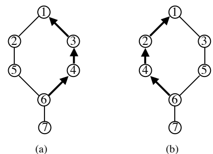
Figure 2: An example topology with two equal-cost paths
