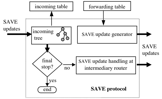
Figure 3: The architecture of the SAVE protocol
