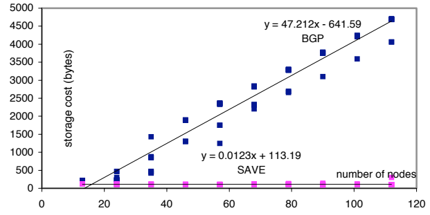
Figure 17: Storage cost for multiple-domain topologies
