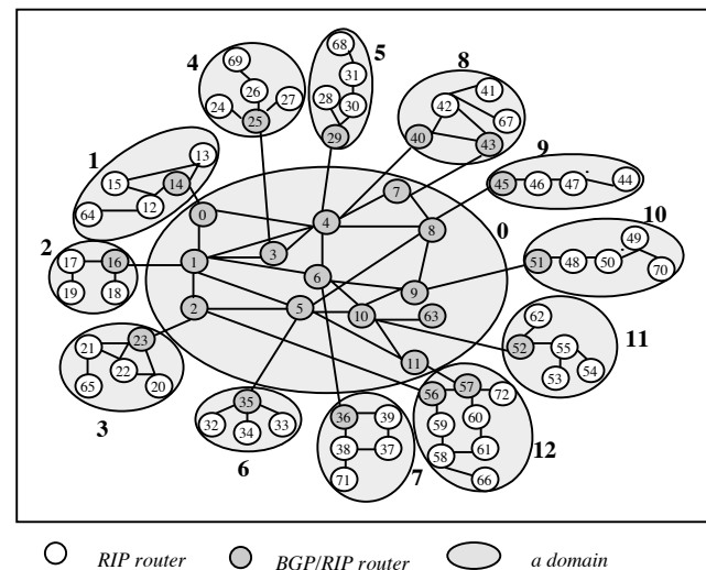
Figure 12: Topology in Experiment 2
