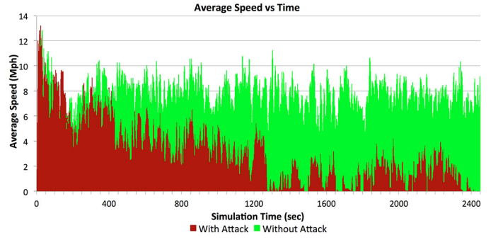
Fig. 3. Average speed on the targeted area with and without active attack
